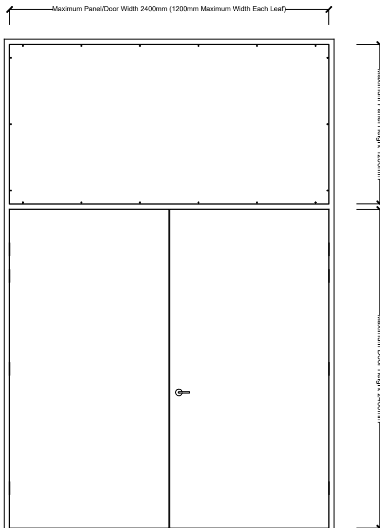
Double Leaf with Transom
