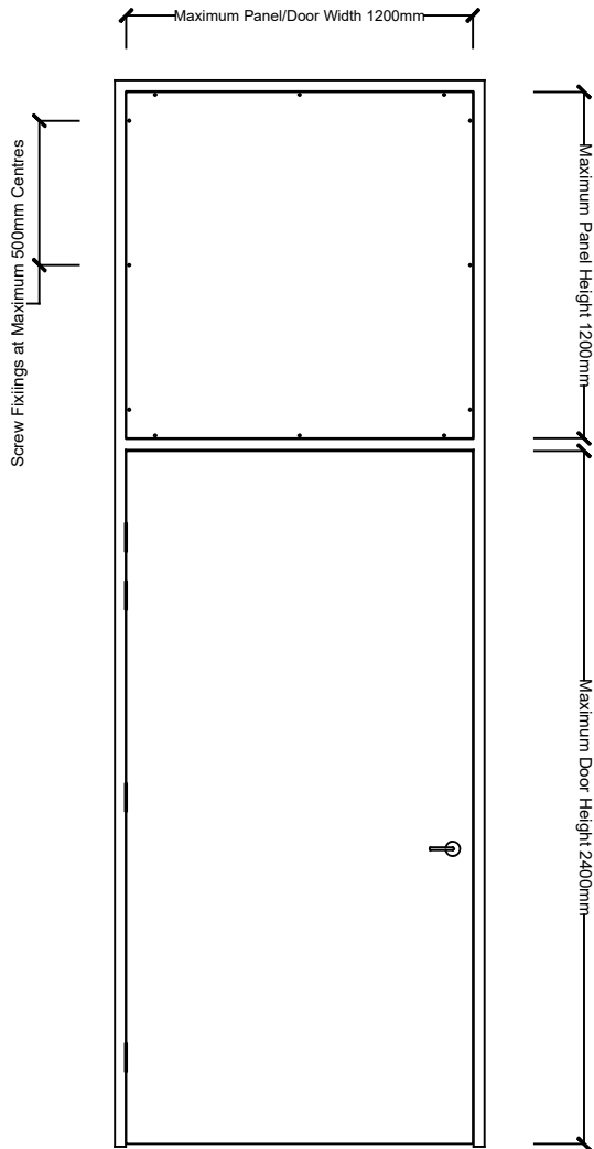
Single Leaf With Transom
