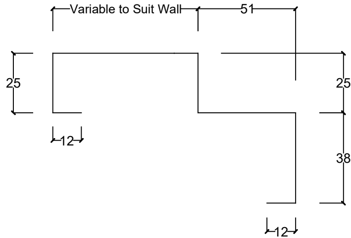
FRAME PROFILE
