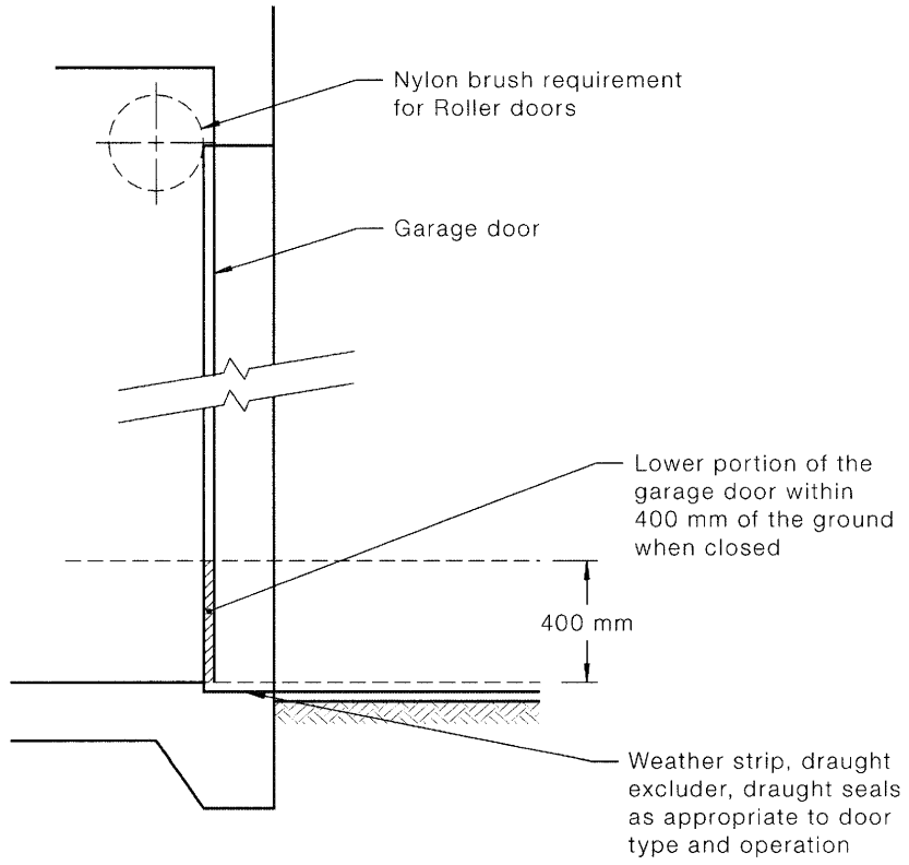
FIGURE D4 VEHICLE ACCESS DOORS (GARAGE DOORS)
