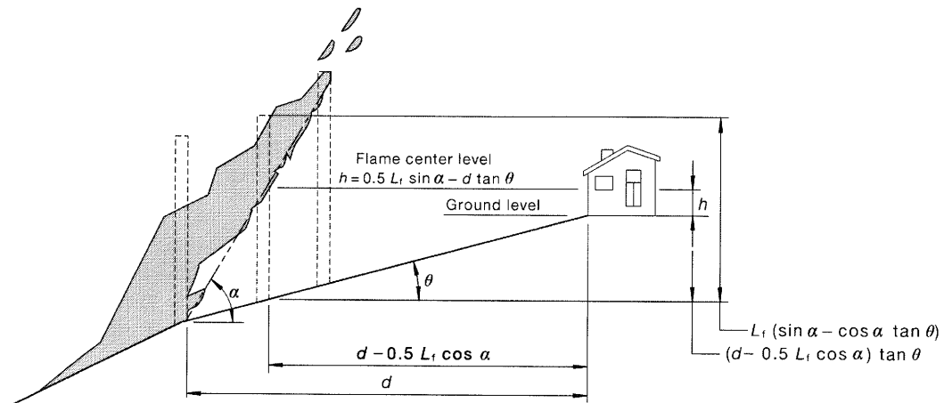
FIGURE B3 FLAME CENTRE HIGHER THAN GROUND
