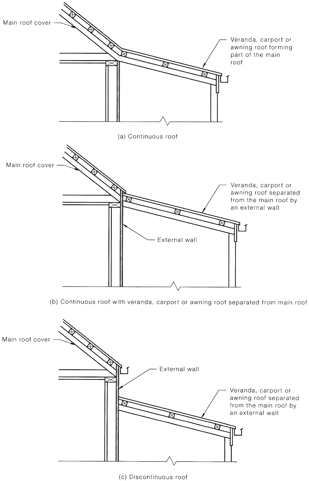
FIGURE D1 VERANDA, CARPORT OR AWNING ROOFS SHOWING CONTINUOUS AND DISCONTINUOUS ROOF TYPES
