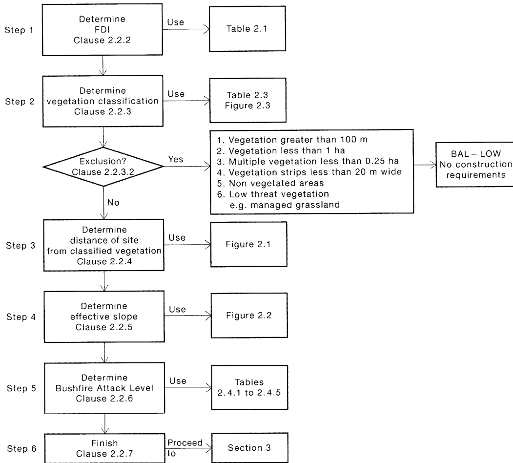
FIGURE C1 DETERMINATION OF THE BUSHFIRE ATTACK LEVEL (BAL)—METHOD 1
