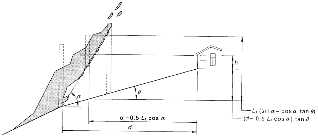
FIGURE B4 DIAGRAM FOR CALCULATING VIEW FACTOR
