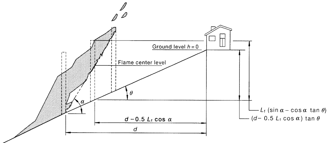
FIGURE B2 FLAME CENTRE LOWER THAN GROUND
