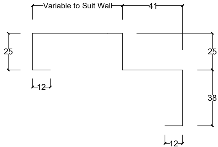
FRAME PROFILE
