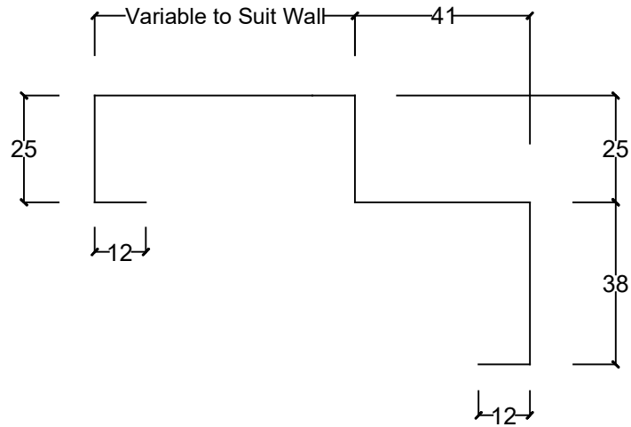
FRAME PROFILE
